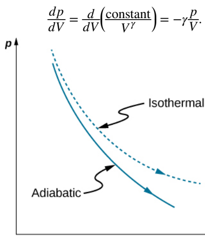
Figure 3.15 Quasi-static adiabatic and isothermal expansions of an ideal gas.
